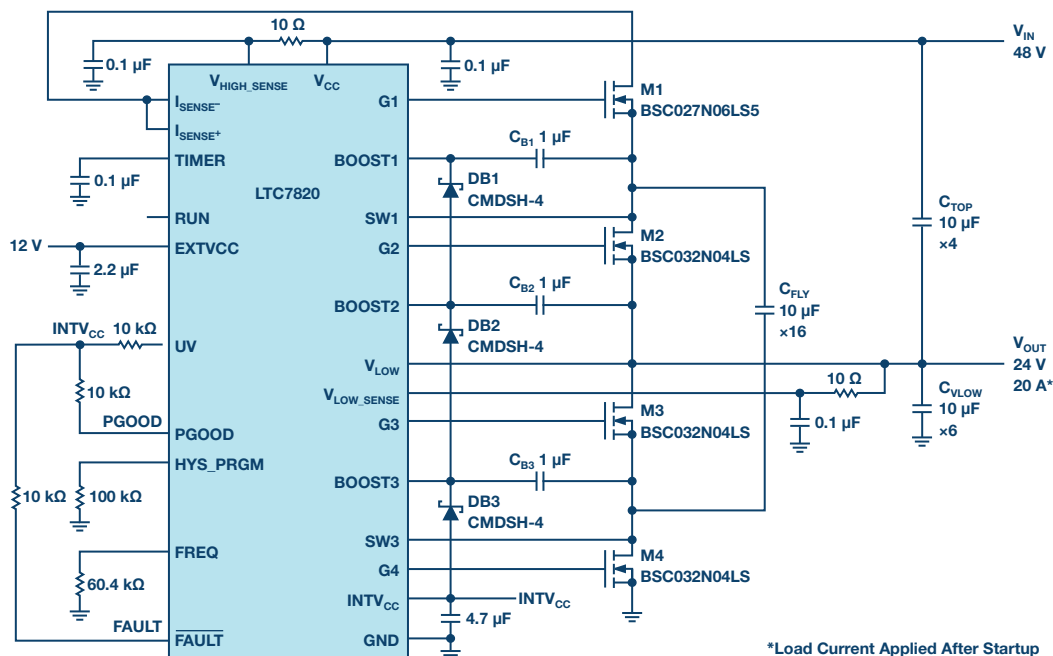
Figure 1. A 48 V to 24 V/20 A voltage divider with a power density of 4000 W/in 2 .
