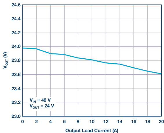
Figure 7. Load regulation.
