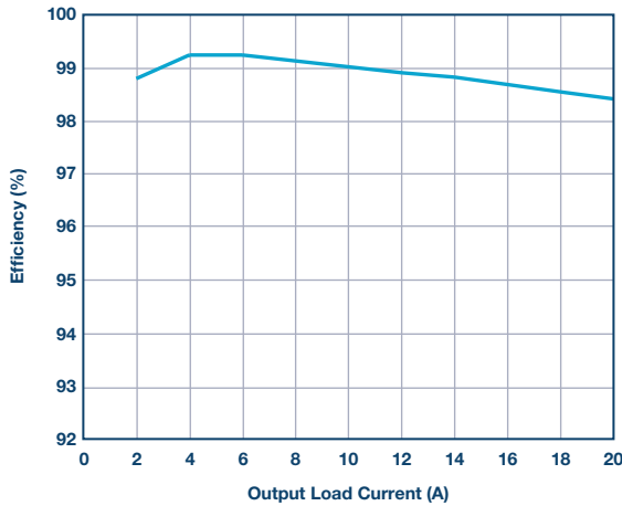
Figure 3. Efficiency at 48 V input, 24 V output, and a 200 kHz switching frequency.
